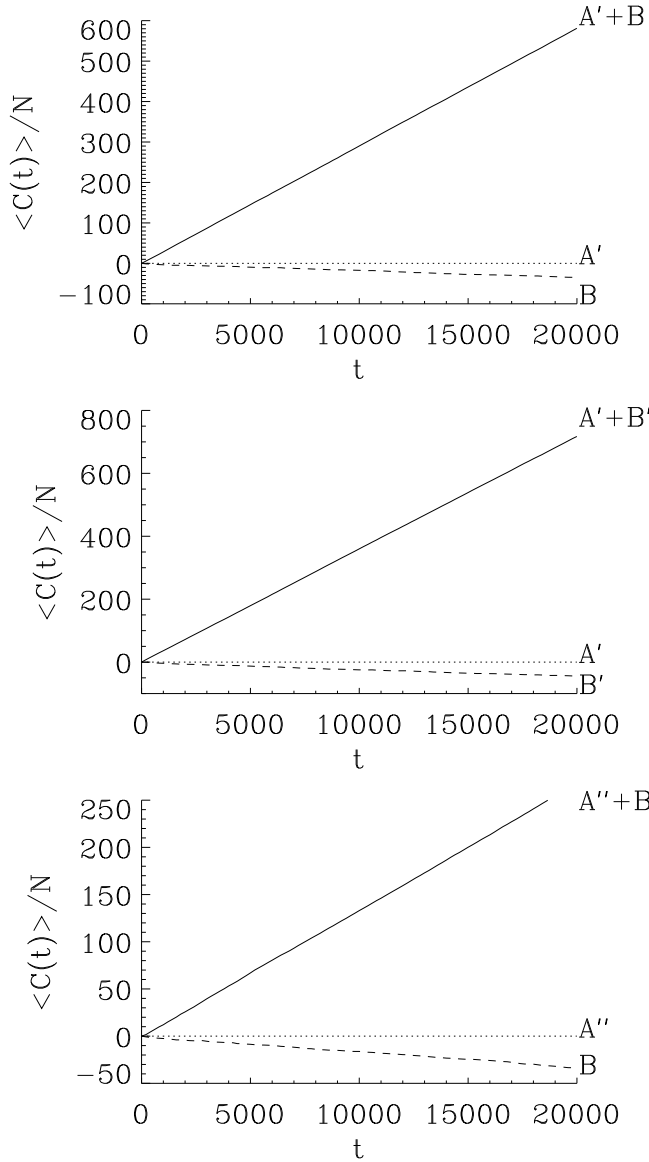
FIG. 1. Average capital per player, \langle C(t) \rangle / N , versus time, t , measured in units of games per player. The different games A' , A'' , B and B' are described in the main text. The probabilities defining the games are as follows: p_1 = 0.1 - \epsilon , p_2 = 0.75 - \epsilon for game B ; p_1 = 0.9 - \epsilon , p_2 = p_3 = 0.25 - \epsilon , p_4 = 0.7 - \epsilon for game B' , with \epsilon = 0.01 in both games. We consider an ensemble of N = 200 players and the results have been averaged for 10 realizations of the games. In all cases, the initial condition is that of zero capital, C_i(0) = 0 , for all players, i = 1, \dots, N . Notice that while games A' and A'' are fair (zero average) and games B and B' are losing games, the random alternation between games as indicated by A'+B (top panel), A'+B' (middle panel) and A''+B (bottom panel) result in winning games.
