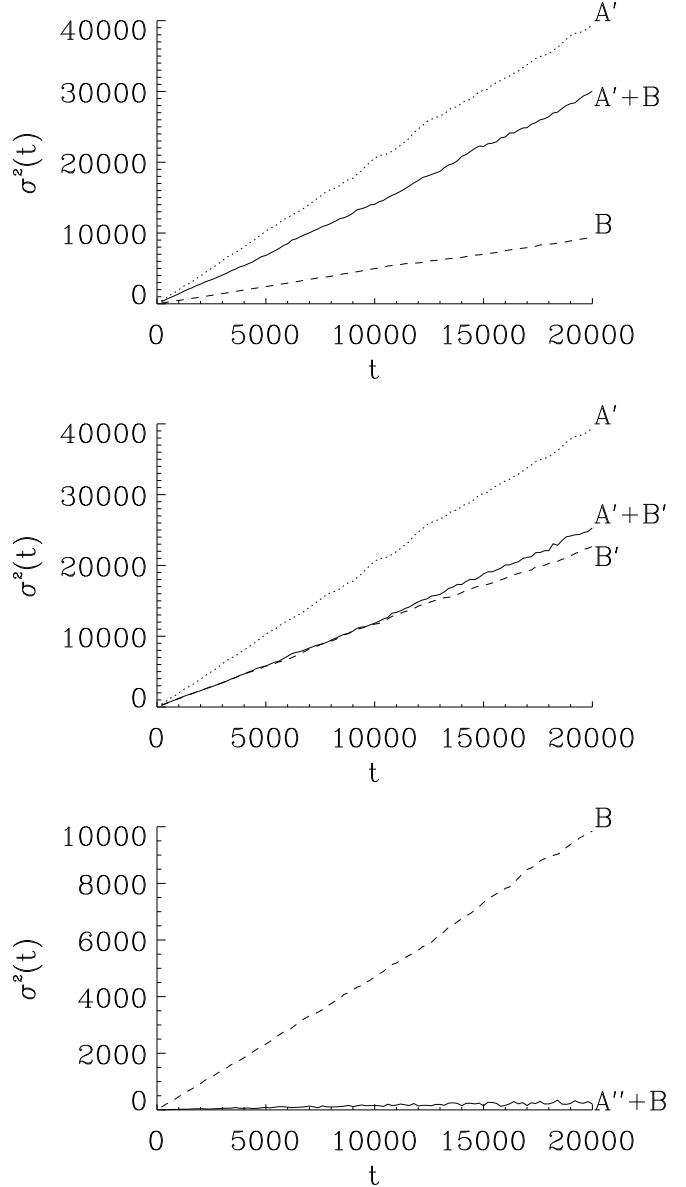
FIG. 2. Time evolution of the variance \sigma^2(t) = \frac{1}{N} \sum_i C_i(t)^2 - \left( \frac{1}{N} \sum_i C_i(t) \right)^2 of the single player capital distribution in the same cases than in figure 1.
